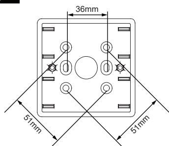
Call Point indoor (Type A)
