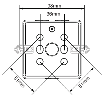
Call Point weatherproof (Type A)
