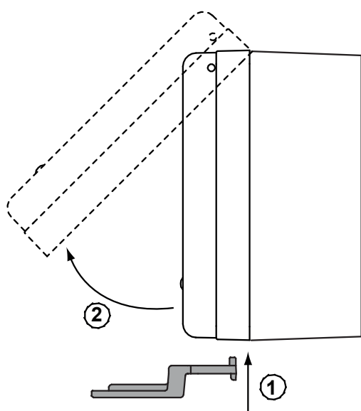
Removing front cover
