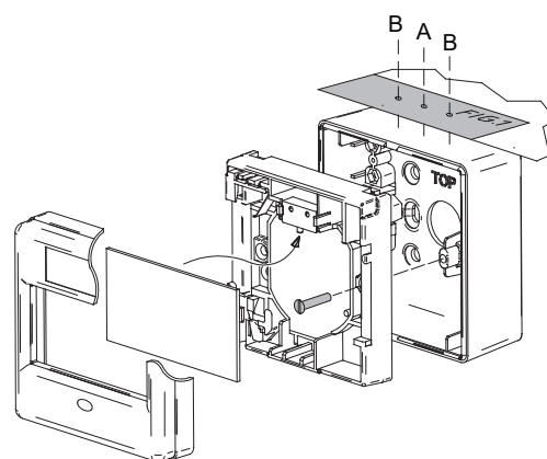
Exploded view (WP)
