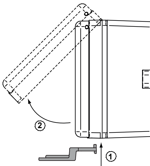
CallPoint weatherproof (WP)
