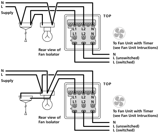
Three pole switching for fan units incorporating timers
