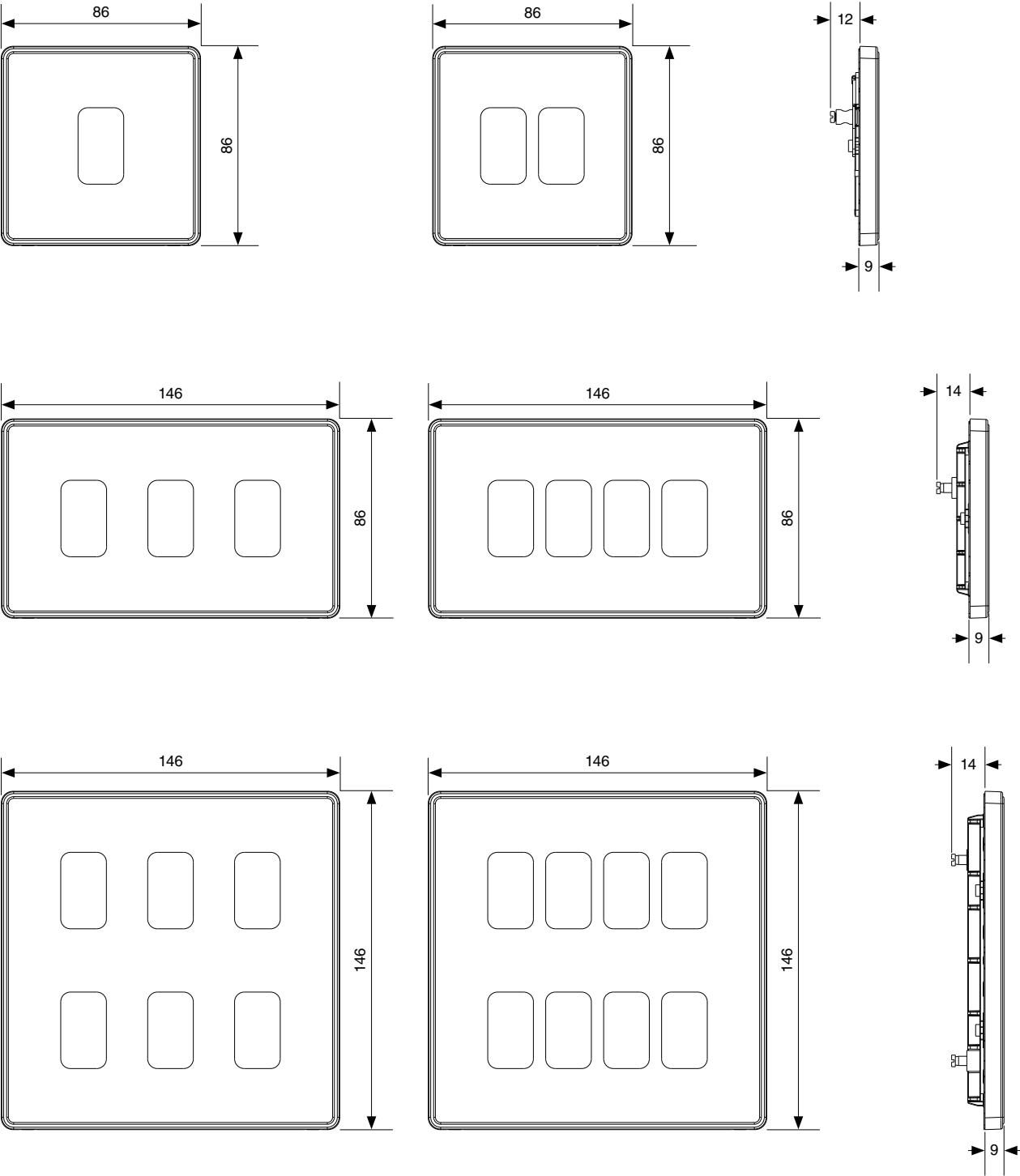
FRONTPLATE DIMENSIONS (MM)
