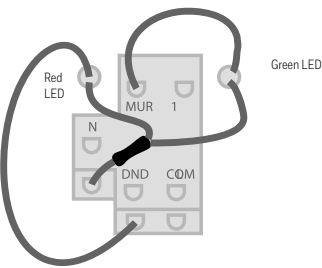
Corridor Switch – Outside “Bell Push/Indicator”
