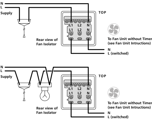
Two pole switching for fan units without timers
