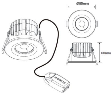
Dimension Diagram
