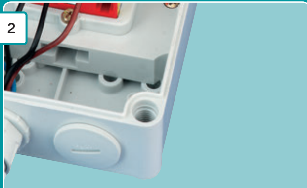
Enclosure fixings outside of sealed enclosure interior to maintain IP rating
