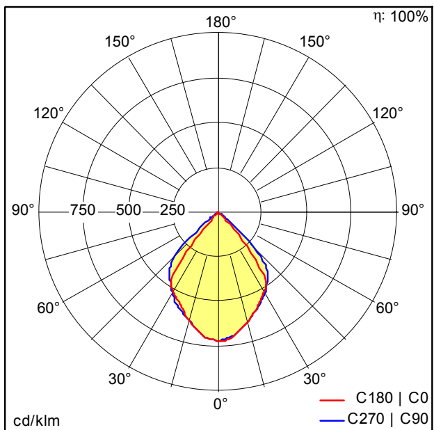
TE_HOLLY_CONE_DOWN_IP65_300_830.idt
