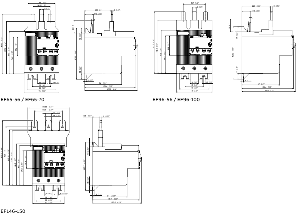
Main dimensions mm, inches
