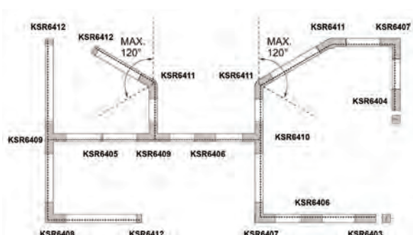
Example Track Layout
