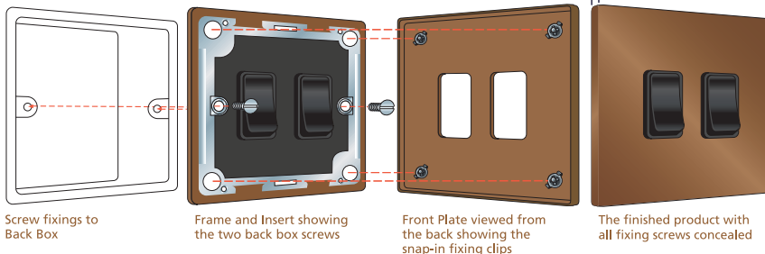
Hamilton Hartland CFX® Bronze Concealed Fixing | Plate depth 5 mm including gasket
