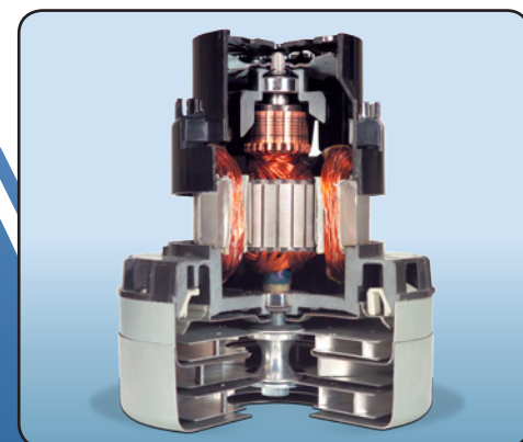
Bypass TwinFlo motor
