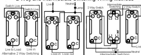
2 Way and Intermediate Switching Wiring Methods
