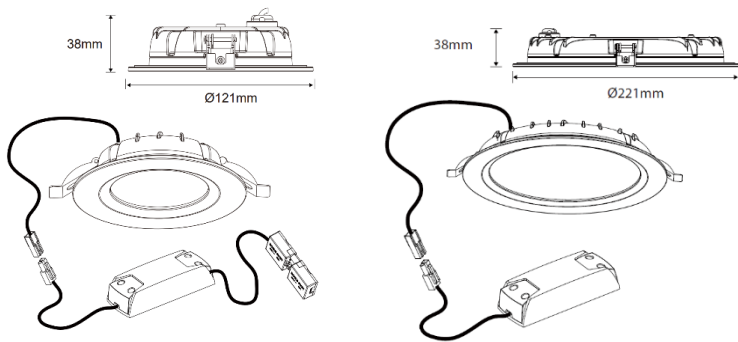
Dimension Diagram
