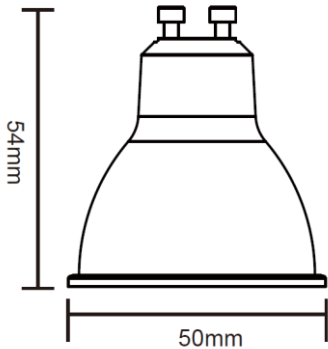
Dimension Diagram
