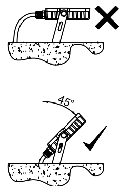
Ground Installation
