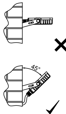
Wall Installation
