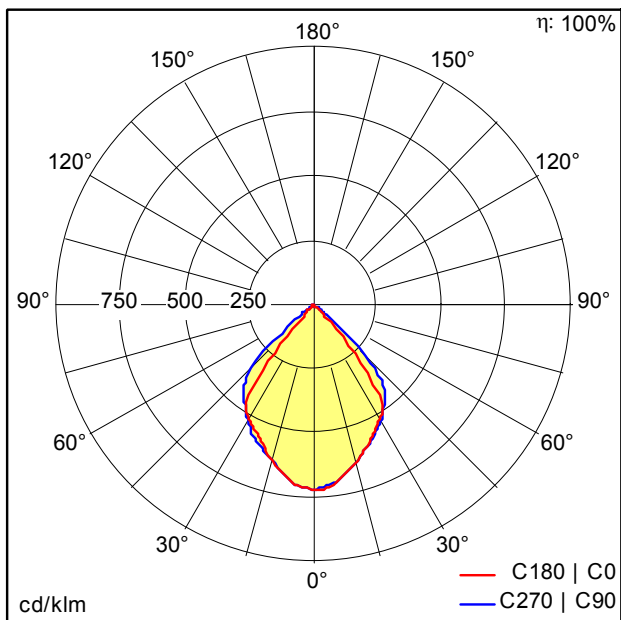
TE_HOLLY_CONE_DOWN_IP65_300_830.ltd
