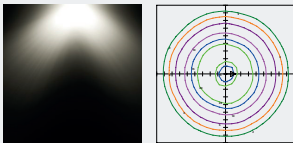
Symmetrical 90° Optic
