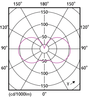
Light Distribution Diagram - MAS LEDBulb DT7.2-75W E27 927A60CL G
