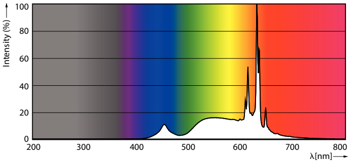
Spectral Power Distribution Colour - MAS LEDBulb DT7.2-75W E27 927A60CL G
