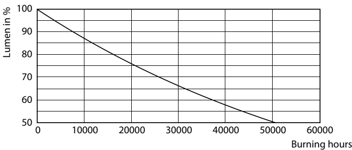
Lumen Maintenance Diagram - MAS LEDBulb DT7.2-75W B22 927A60CL G
