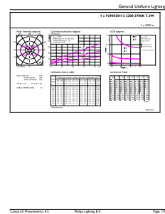
General uniform lighting - MAS LEDBulb DT7.2-75W B22 927A60CL G
