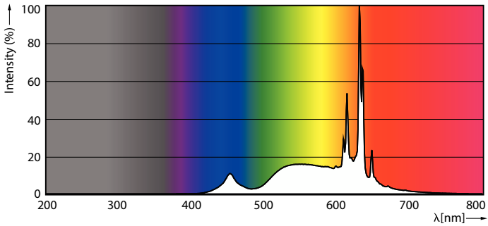
Spectral Power Distribution Colour - MAS LEDBulb DT7.2-75W B22 927A60CL G
