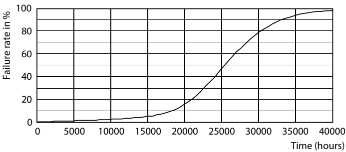
Life Expectancy Diagram - MAS LEDBulb DT7.2-75W B22 927A60CL G
