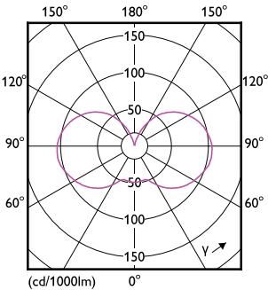
Light Distribution Diagram - MAS LEDBulb DT7.2-75W B22 927A60CL G
