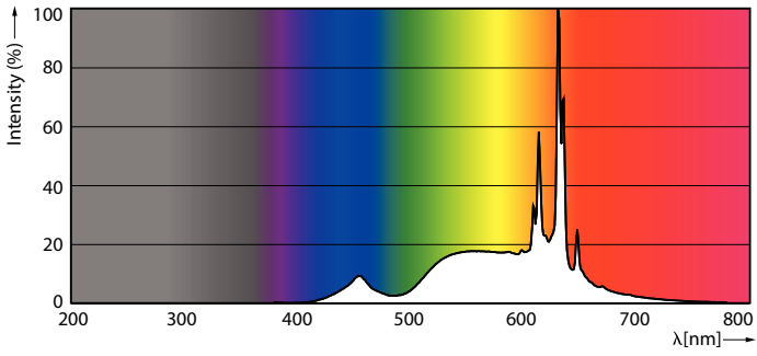
Spectral Power Distribution Colour - MAS LEDBulbDT10.5-100W B22 927A60CLG
