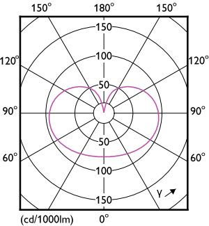
Light Distribution Diagram - MAS LEDBulbDT10.5-100W B22 927A60CLG
