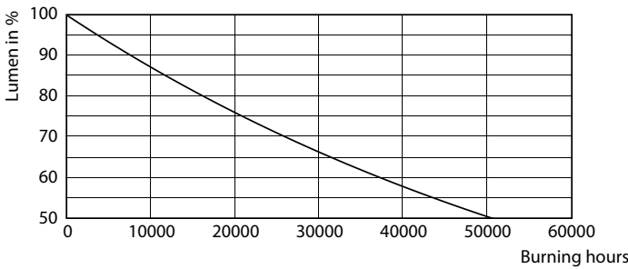
Lumen Maintenance Diagram - MAS LEDBulbDT10.5-100W B22 927A60CLG
