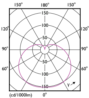
Light Distribution Diagram - CoreProLEDbulb ND 4.9-40W A60 B22 927 UK
