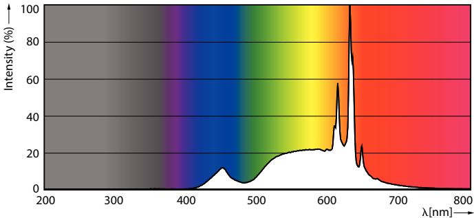
Spectral Power Distribution Colour - CoreProLEDbulb ND 4.9-40W A60 B22 927 UK
