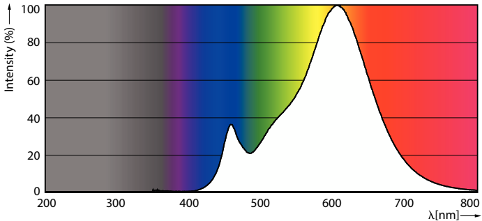
Spectral Power Distribution Colour - CoreProLEDbulb ND 13-100W A60 B22 927 UK
