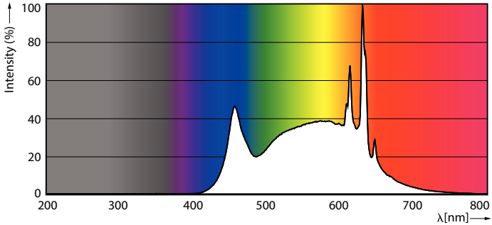
Spectral Power Distribution Colour - CorePro LEDbulb ND 7.5-60W A60 E27 940UK
