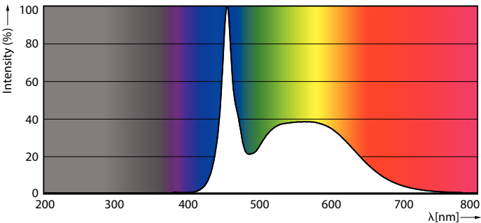
Spectral Power Distribution Colour - CorePro LEDtube 1800mm 21W 865 T8
