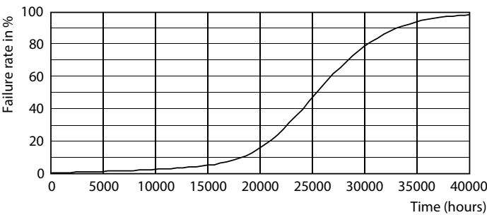
Life Expectancy Diagram - MAS LEDCandleDT3.4-40W E27 927 B35CL G
