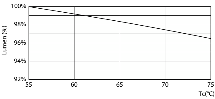
Lumen Maintenance Diagram - MAS LEDtube 1500mm UO 36W 840 T5
