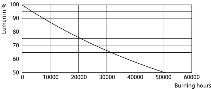
Lumen Maintenance Diagram - MAS LEDBulbDT5.9-60WB22 927A60CL G UK
