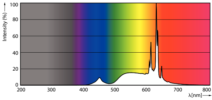
Spectral Power Distribution Colour - MAS LEDBulbDT5.9-60WB22 927A60CL G UK
