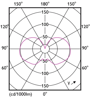
Light Distribution Diagram - MAS LEDBulbDT5.9-60WB22 927A60CL G UK
