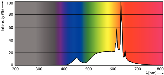
Spectral Power Distribution Colour - CoreProLEDbulb ND 4.9-40W A60 E27 927 UK
