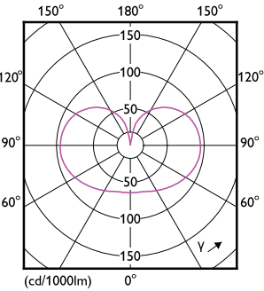
Light Distribution Diagram - MASVLE LEDBulbD5.9-60W B22A60 927FR G UK
