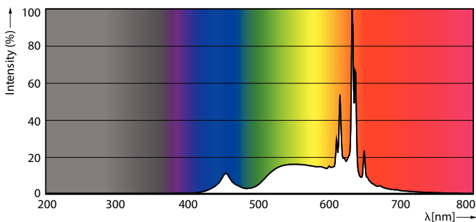
Spectral Power Distribution Colour - MAS VLE LEDBulbD7.2-75W B22 A60 927 FR G
