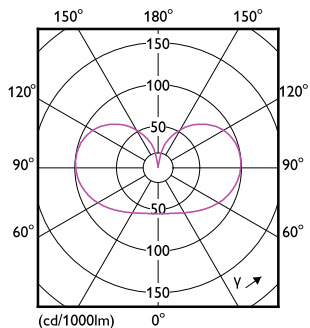
Light Distribution Diagram - MAS VLE LEDBulbD7.2-75W B22 A60 927 FR G
