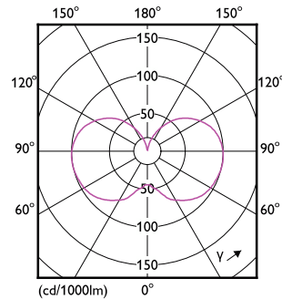
Light Distribution Diagram - MASVLE LEDBulbD10.5-100W B22A60 927FRGUK
