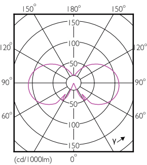
Light Distribution Diagram - CoreProLEDCandleND4.3-40WE14 827B35CLGUK
