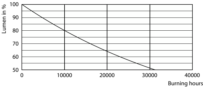
Lumen Maintenance Diagram - CoreProLEDCandleND4.3-40WE14 827B35CLGUK
