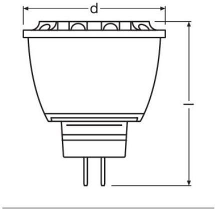
P MR11 20 30° 3.1 W/2700K GU4
