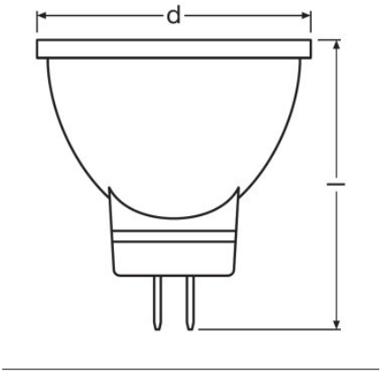
P MR11 20 36° 2.6 W/2700K GU4, P MR11 35 36° 4 W/2700K GU4
