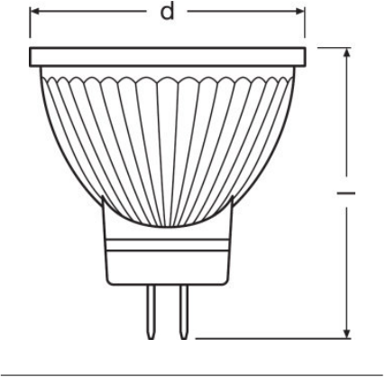
P MR11 20 36° 3.2 W/2700K GU4, P MR11 35 36° 4.5 W/2700K GU4
