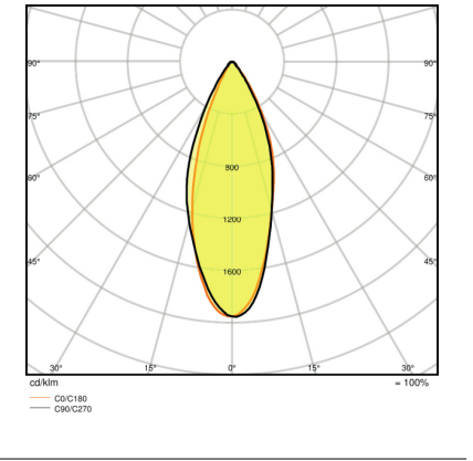
P MR11 20 36° 2.6 W/2700K GU4, P MR11 20 36° 3.2 W/2700K GU4
