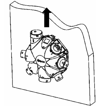
In the vertical position: The outlet must face vertically
