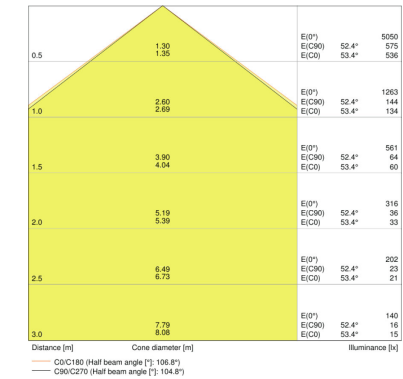
DL ALU DALI DN 200 35 W 4000 K IP44 WT
