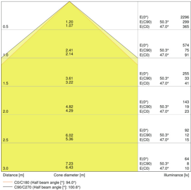
DL ALU DALI DN 150 14 W 3000 K IP44 WT
