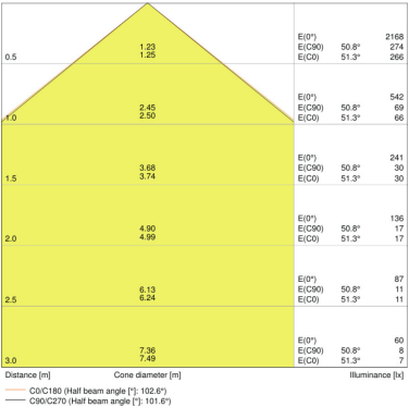
DL ALU DALI DN 150 14 W 4000 K IP44 WT
