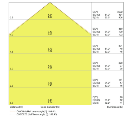
DL ALU DALI DN 200 25 W 3000 K IP44 WT
