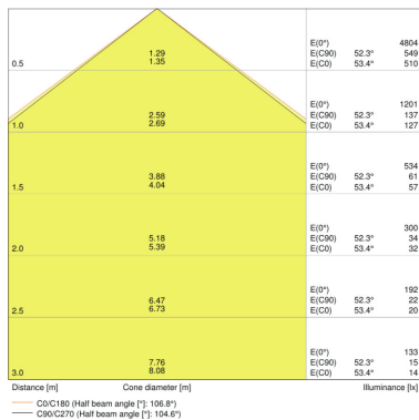
DL ALU DALI DN 200 35 W 3000 K IP44 WT
