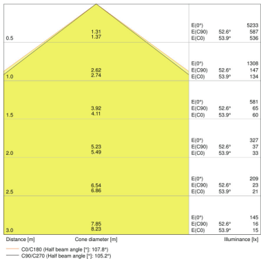
DL ALU DALI DN 200 35 W 6500 K IP44 WT
