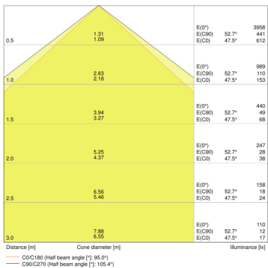
DL ALU DALI DN 200 25 W 4000 K IP44 WT
