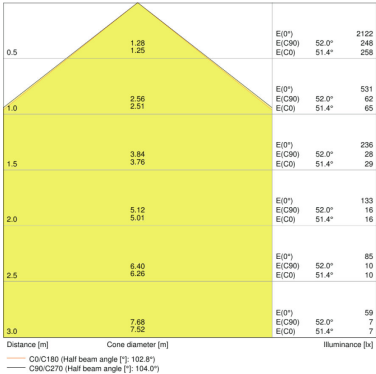
DL ALU DALI DN 150 14 W 6500 K IP44 WT
