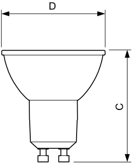
GU10 4-50W 370lm 4000K GU10 D 15khrs
