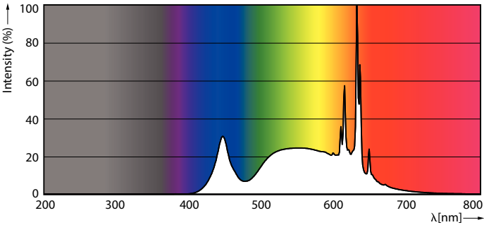
LEDspots Corepro SLR 4W PAR16 GU10 840 36D-POC
