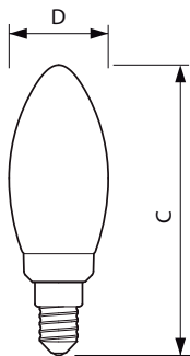
Candle B35 EU 2-25W 270lm WG E14 CL
