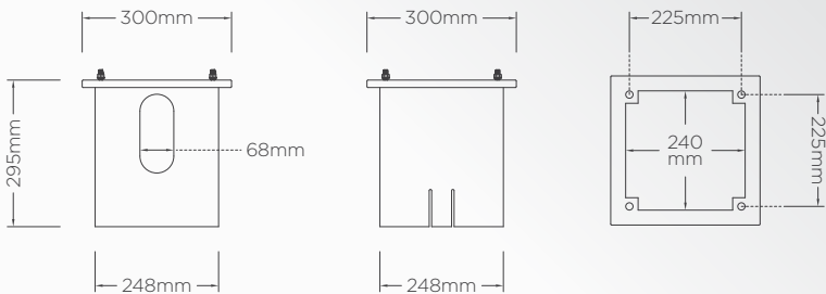
Ground mounting base
