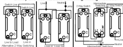
2 Way and Intermediate Switching Wiring Methods
