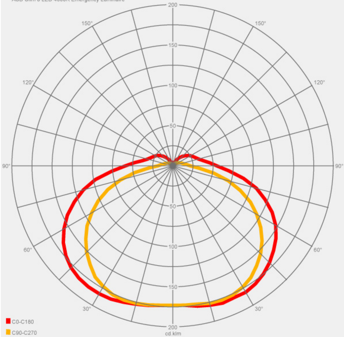
ASD Slim 8 LED 4000K Emergency Luminaire
