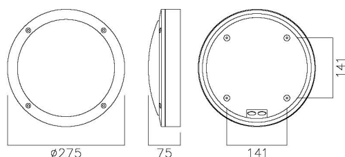
PLAIN TRIM
