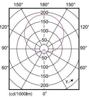
CorePro LEDbulb ND 10-75W A60
