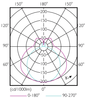
LEDtube PLC 400mm 16-5W 2G11 830 2000lm
