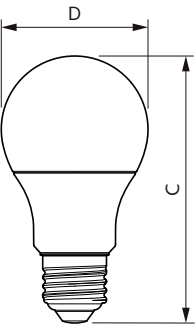
Bulb A60S+ 230V 8.5-60W 806lm 2700K E27
