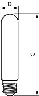
TForce 40W 7000lm 3000K E40 ND
