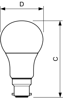
Entrybulb 230V 10.5W-75W 2700K B22 ND
