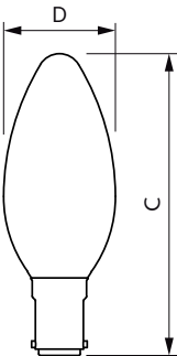
Candle B35 EU 3.5-40W 475lm WG B15 CL
