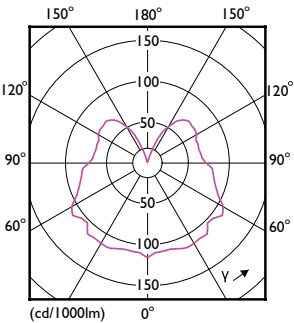
LEDbulb MAS SLR1 A60 5,5W B22 827 CL-LDD
