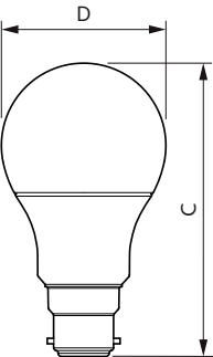
MASTER LEDbulb DT 5.5-40W B22 A60 CL
