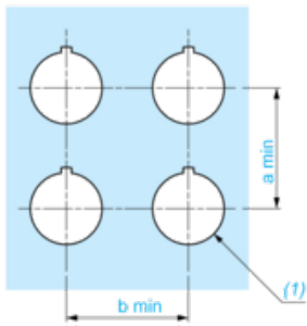
(1) Diameter on finished panel or support
