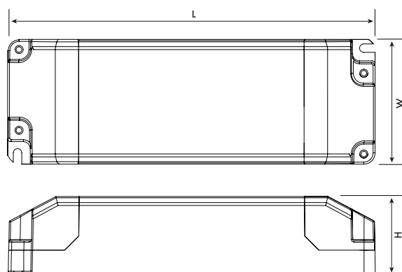
PCV20 Series 20W Driver Mechanical
