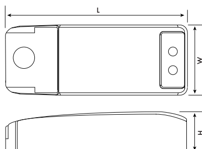
PCV12 12W Series Driver Mechanical
