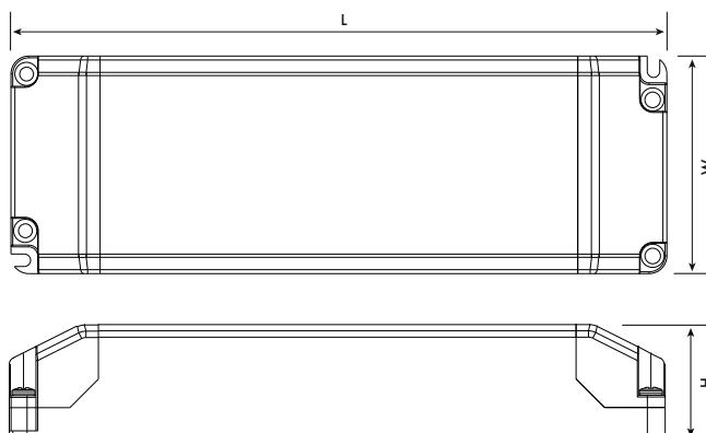
PCV36 & PCV50 Series 36W & 50W Drivers Mechanical
