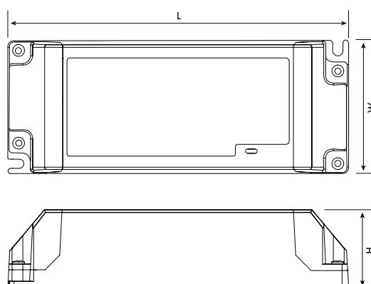
PCV60 Series 60W Driver Mechanical
